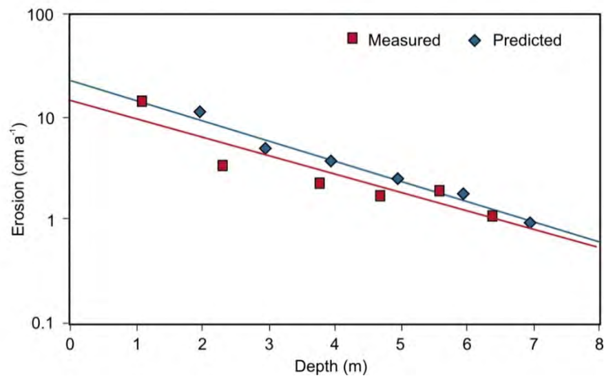
Figure 7: Comparison of measured average annual vertical erosion rates at Grimsby, Lake Ontario with rates predicted from equation 1 and measured average annual bluff recession rate of 1.1 m/y. (Davidson-Arnott, 2010, Fig. 13.16)
