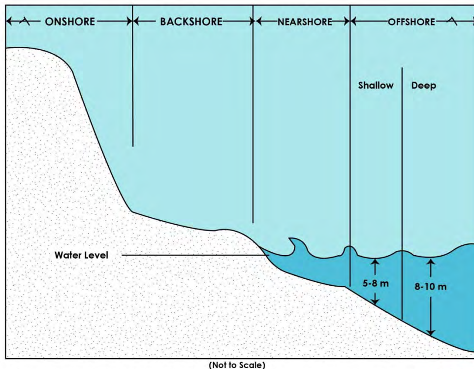
Figure 1 – Definition of Shoreline Zone. Note that the transition from the nearshore to the offshore is defined by the breaker line in this diagram but in the body of the paper it is defined by the limit of wave action on the bed which is about 10-12 m on the ABCA coast.
