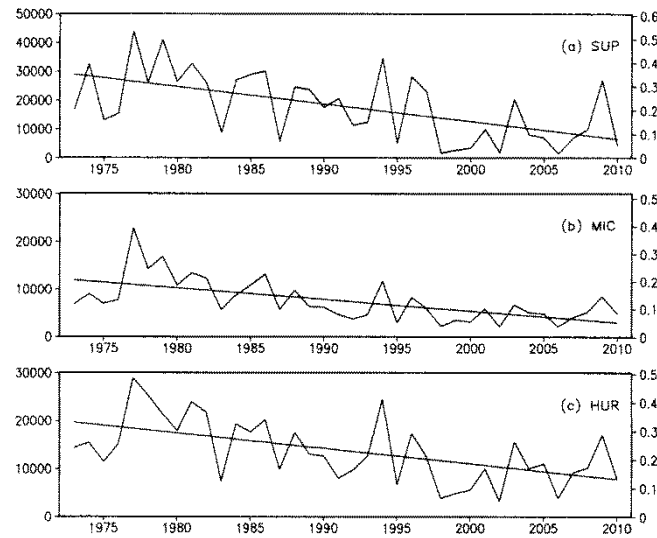
Figure 3: Annual mean lake ice area ( \text{km}^2 ) for Lakes Superior, Michigan and Huron for the period 1973-201 and least squares trend line (from Wang et al., 2012, Figure 5).
