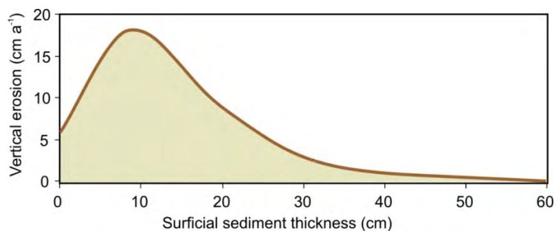
Figure 8: Hypothetical relationship between average surficial sediment cover on the cohesive profile versus average rate of downcutting. The scales are intended to suggest the order of magnitude relationship for a point in shallow water. Note that some erosion will continue underwater in places even with quite thick sediment cover because the sediment is not distributed uniformly (Davidson-Arnott, 2010 – Figure 13.19).
